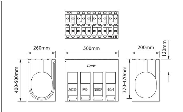
Canal ACO Drain RoadDrain® 200, 0,5 m
